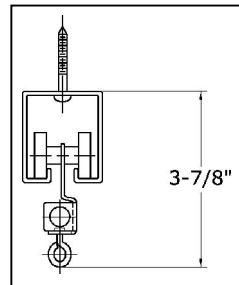
Cross Section of 170 Ceiling Mount
