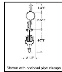
Cross Section of 142 Track Pipe Mounted
